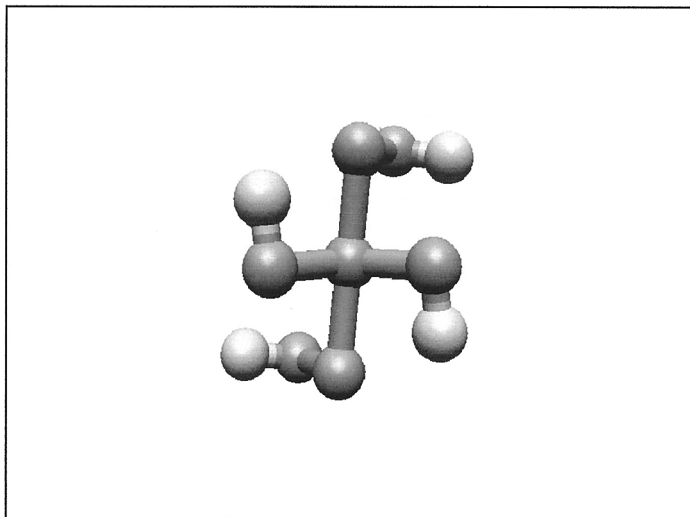
Fig. 1: A representative molecule, \text{H}_4\text{S}_7 , containing a hypervalent sulfur atom. The geometry of the molecule is pseudo-trigonal bipyramid, with a lone pair occupying one of the three equatorial sites.
